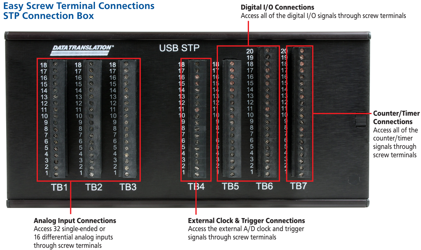
Figure 3. The STP connection box is available for easy signal connections on the 32-channel version of the module
