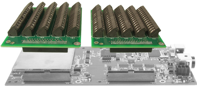
Figure 7. The EP355 screw terminal panel plugs into the J2 or J3 connector on the OEM version of the DT9844 module.
