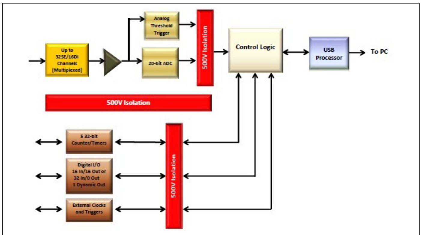
Figure 2. The block diagram of the DT9844 shows the \pm 500V isolation between three subsystems and the host computer. All circuitry is designed to preserve the lowest noise for analog data acquisition.
