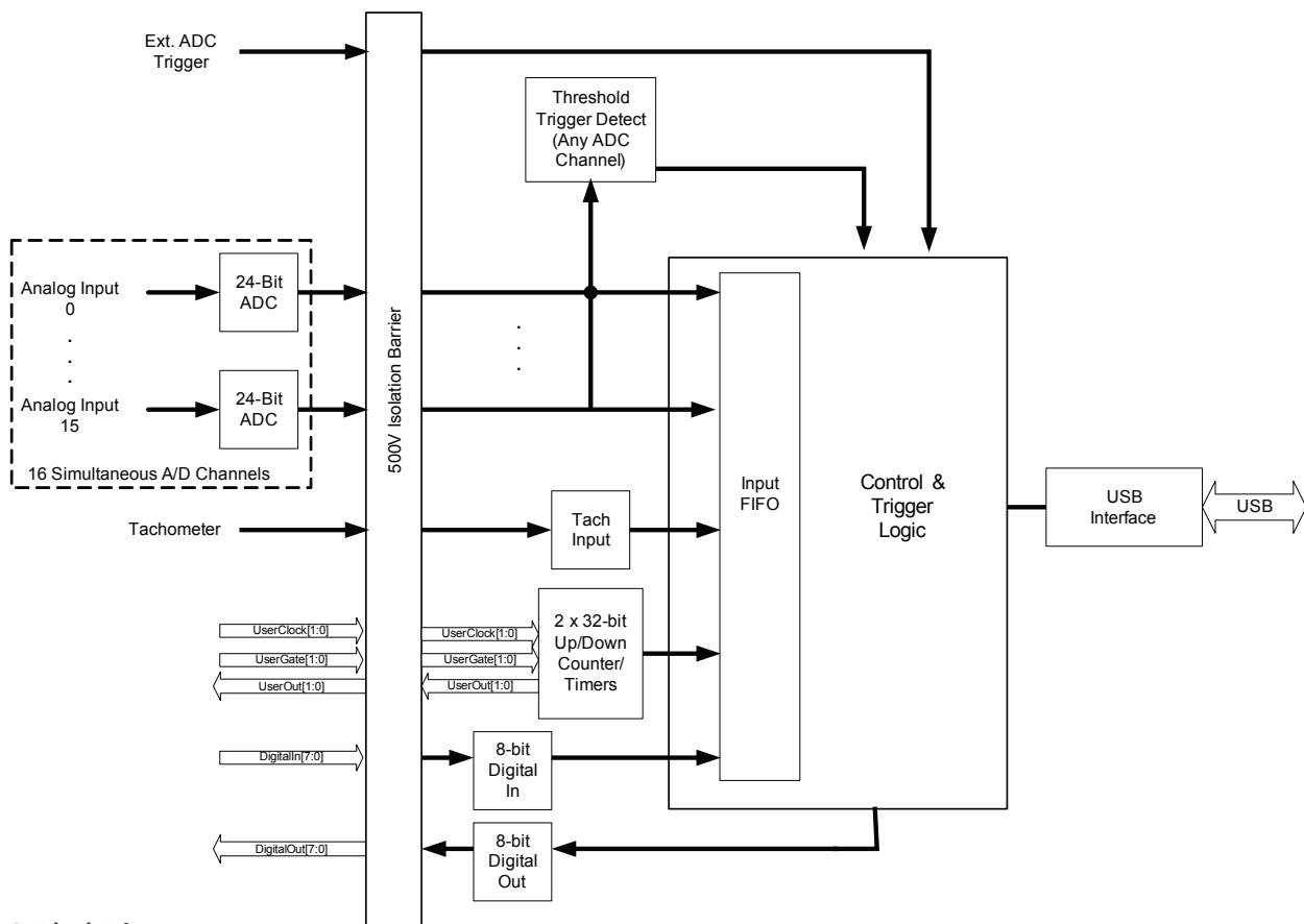
Figure 2. Block Diagram.
