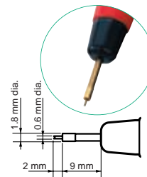
9770 PIN TYPE LEADS (Cable length: connector to fork 40 cm, fork to probes 25 cm)
